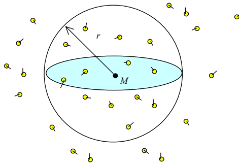
Figure 12: Nearest photons
