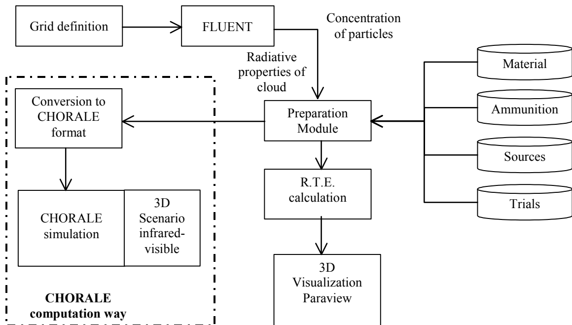
Figure 6: Architecture of simulation
