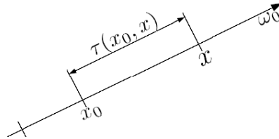
Figure 10: Geometry associated to the volume transfer equation
