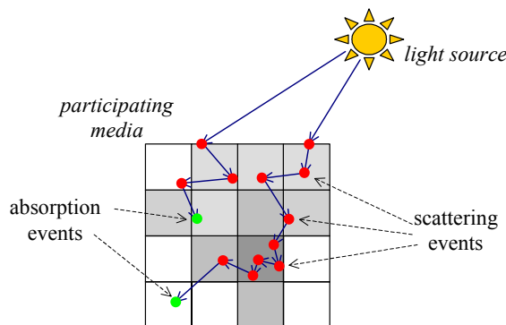
Figure 11: Photons propagation
