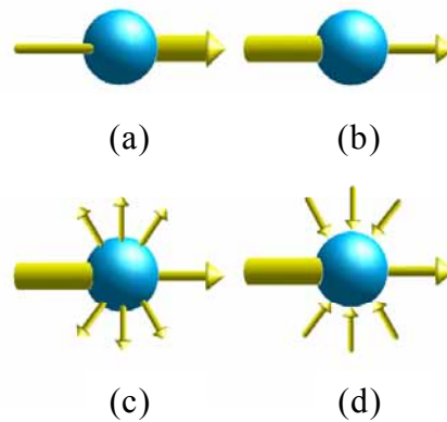
Figure 9: Phenomena affecting light propagation. (a) Emission.(b) Absorption. (c) Out-scattering. (d) In-scattering.
