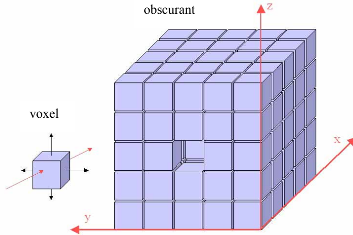
Figure 7: Obscurant representation using voxels
